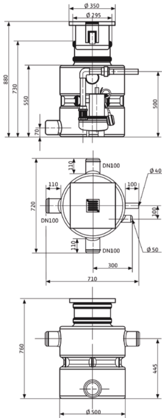
Wilo-DrainLift Box 40
