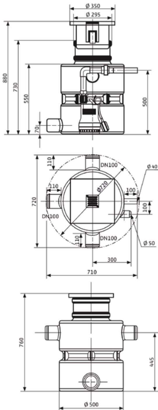
Wilo-DrainLift Box 32
